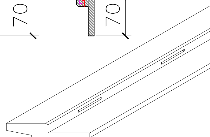
Isometric
