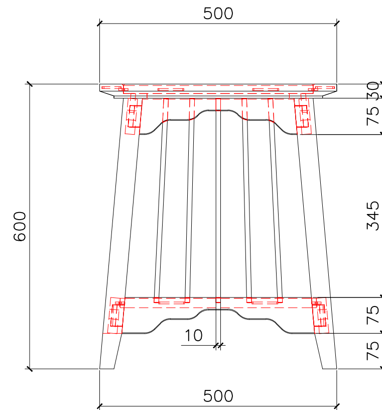
Side view Scale 1:100
