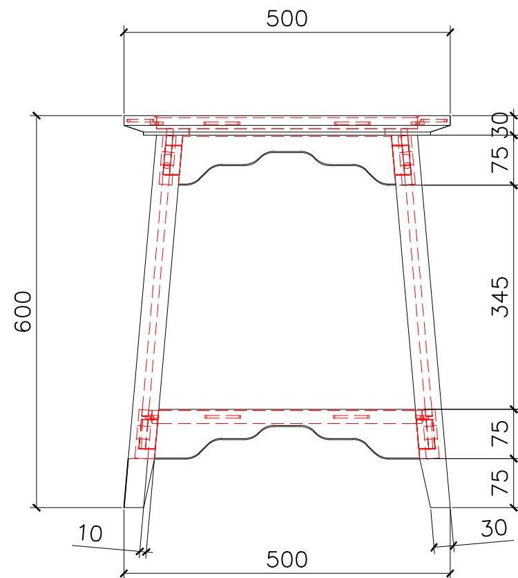
Front view Scale 1:100
